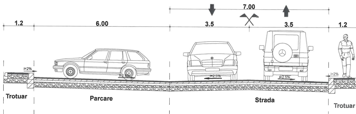
Section 2-2
