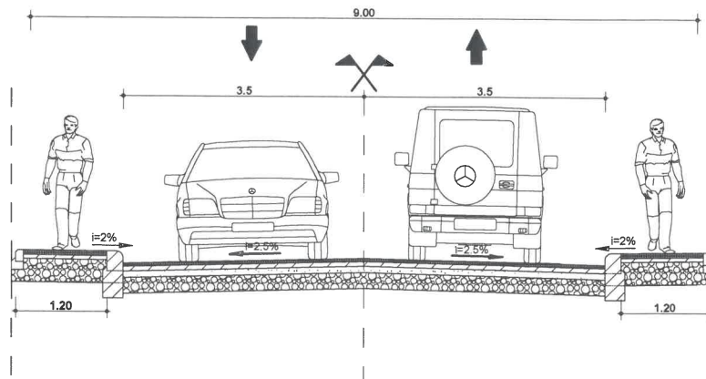
Section 1-1
